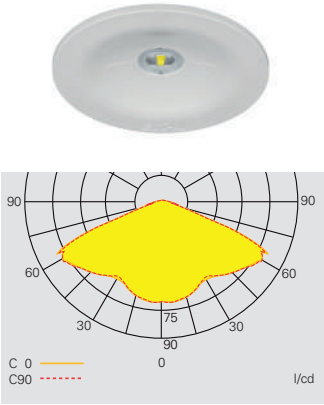
Light distribution curve GuideLed SL 13021.2 CG-S recessed with symmetric optics
