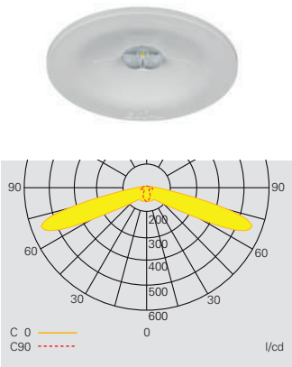
Light distribution curve GuideLed SL 13011.2 CG-S recessed with asymmetric optics
